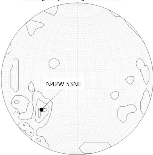
Cu-bearing and Pyrite-bearing Veins and Veinlets
