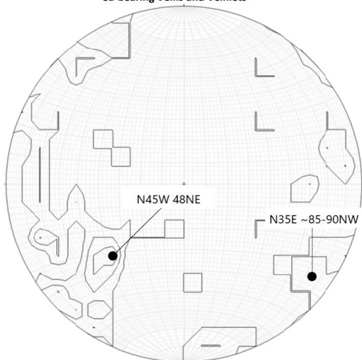
Cu-bearing Veins and Veinlets
